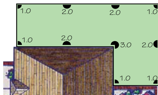
AREA C = 16 GPM PGJ MID-RANGE ROTORS
